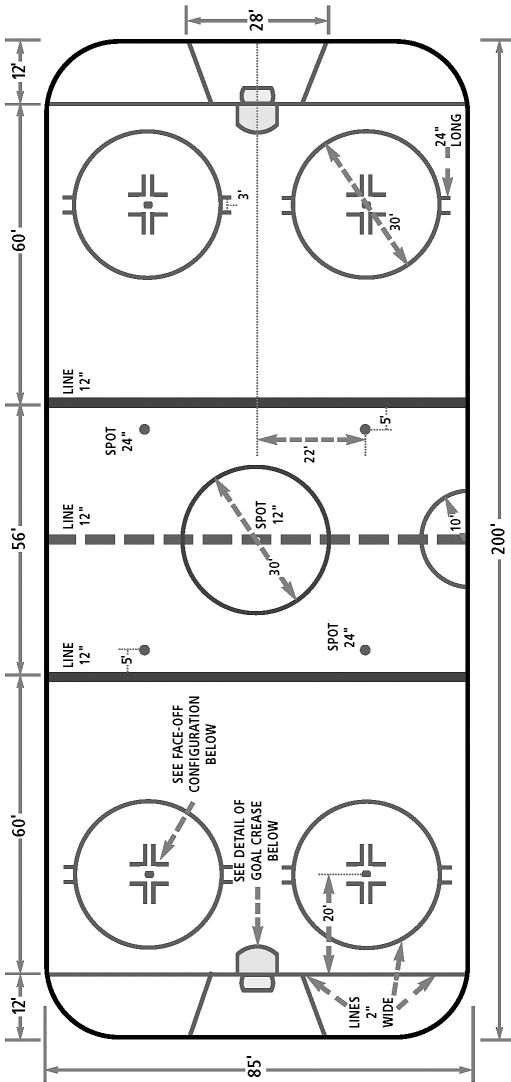
OFFICIAL DIMENSIONS OF RINK SURFACE
